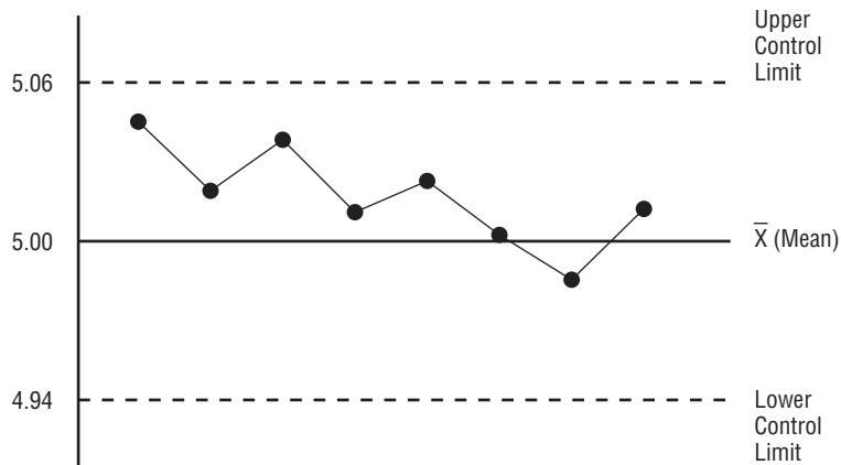
FIGURE 11.2 Control chart
